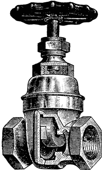
Weber's Gate Valve.
